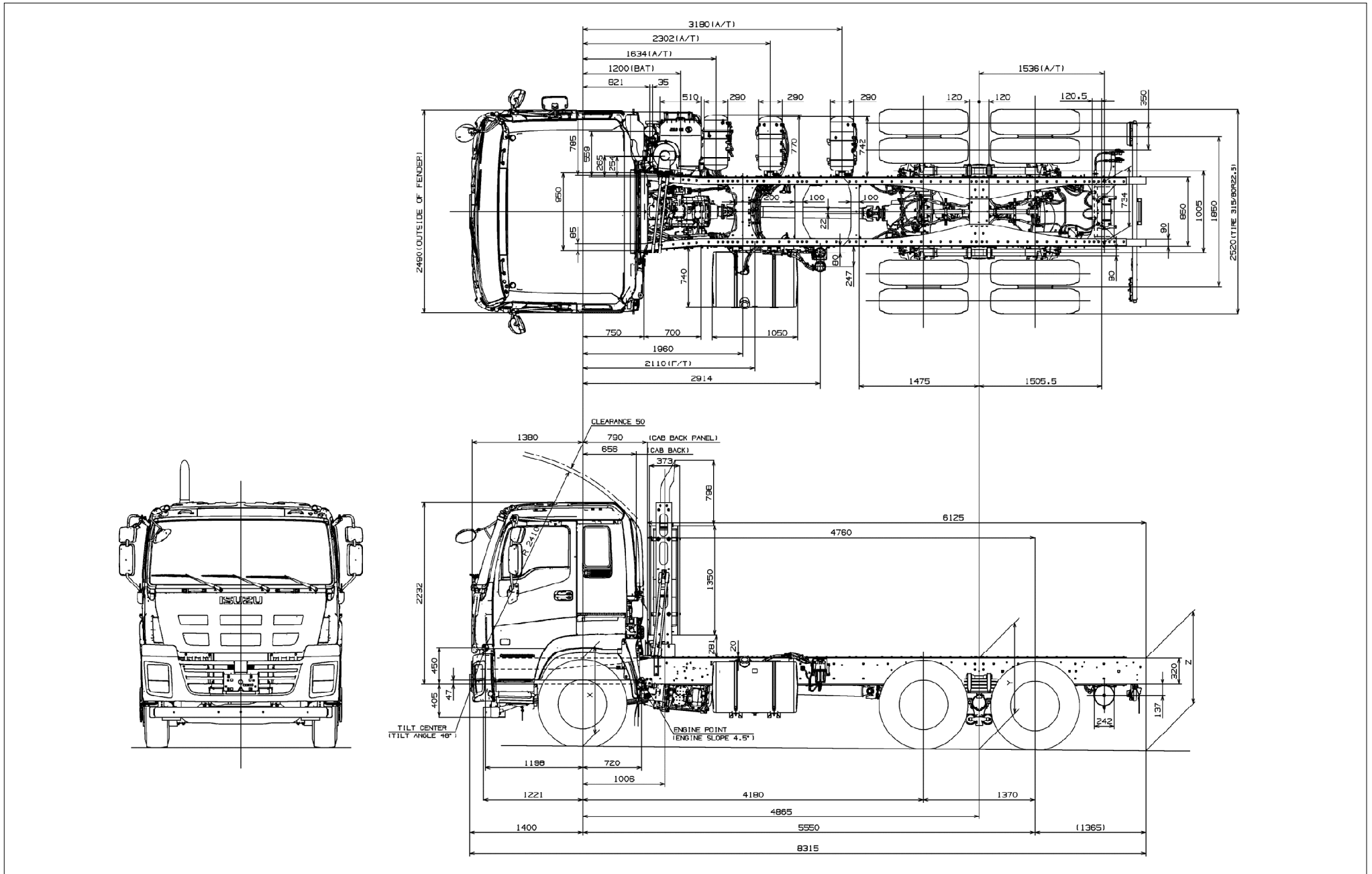
Fig. 9-1-4 Cab Chassis Drawing CYZ52PLD3T17 (T/M: MJT7S)
