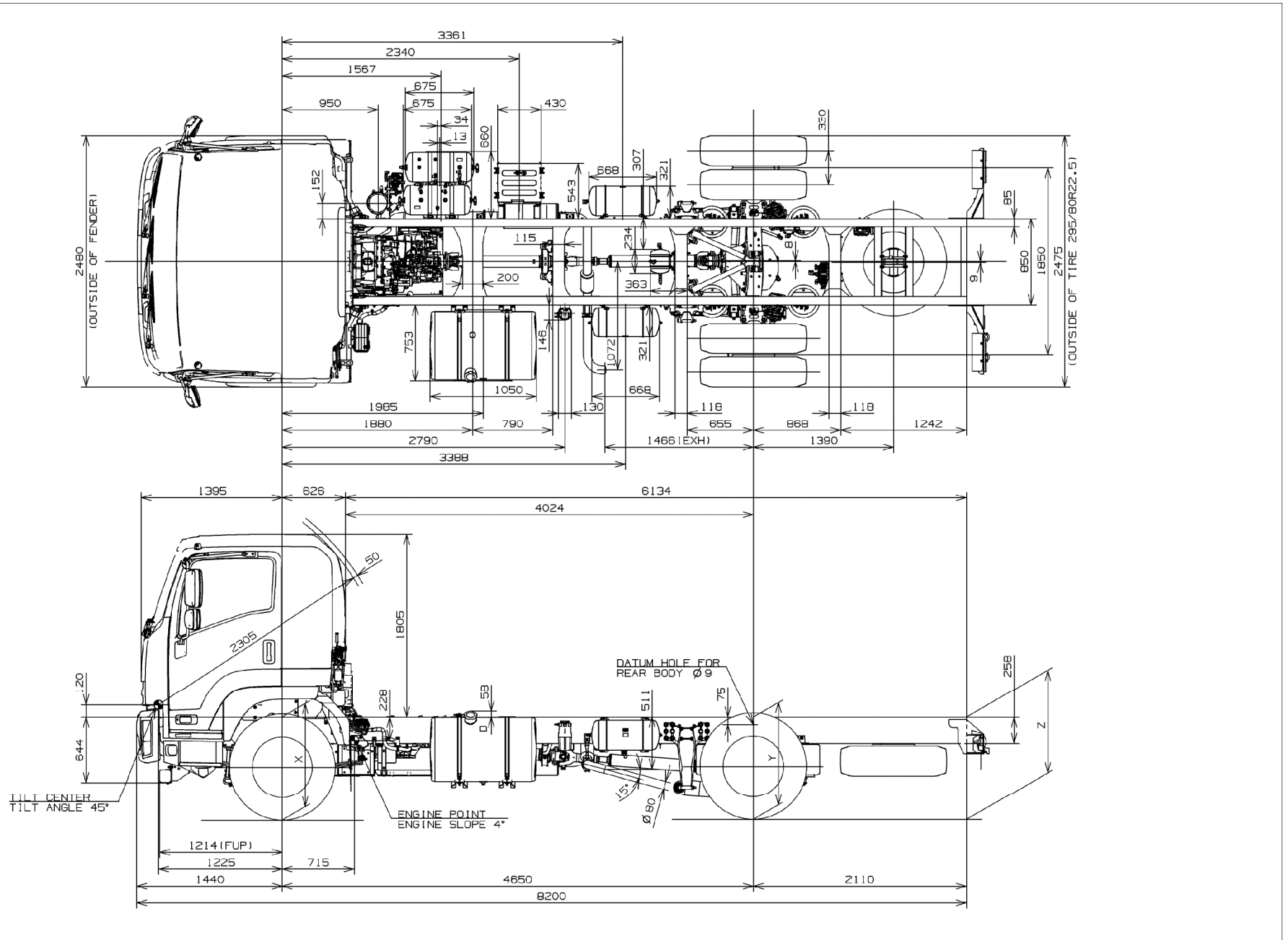
Fig. 9-1-9 Cab Chassis Drawing FVR34VL-MDUC
