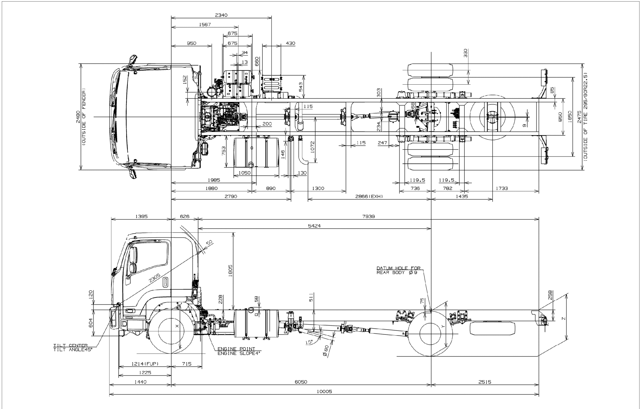
Fig. 9-1-8 Cab Chassis Drawing FVR34UL-SDUC
